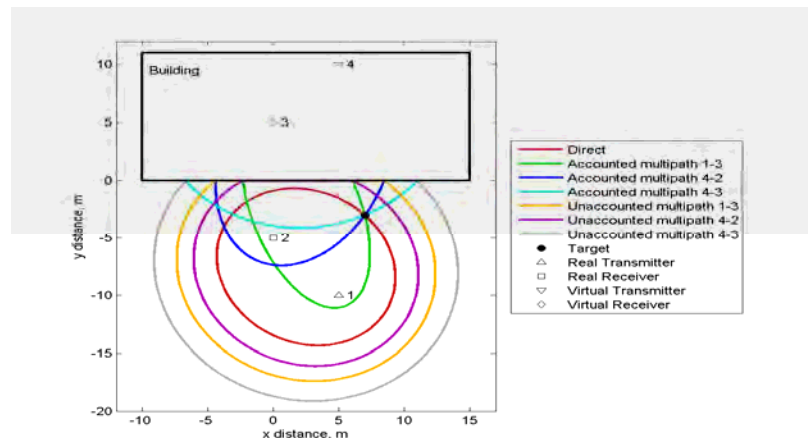
FIGURE 4. Target detection using one transmitter and one receiver, in the presence of multipath caused by a building
