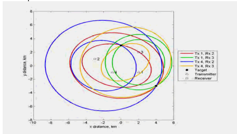
FIGURE 2. Ellipse geometry for a two-target scenario with two transmitters and two receivers
