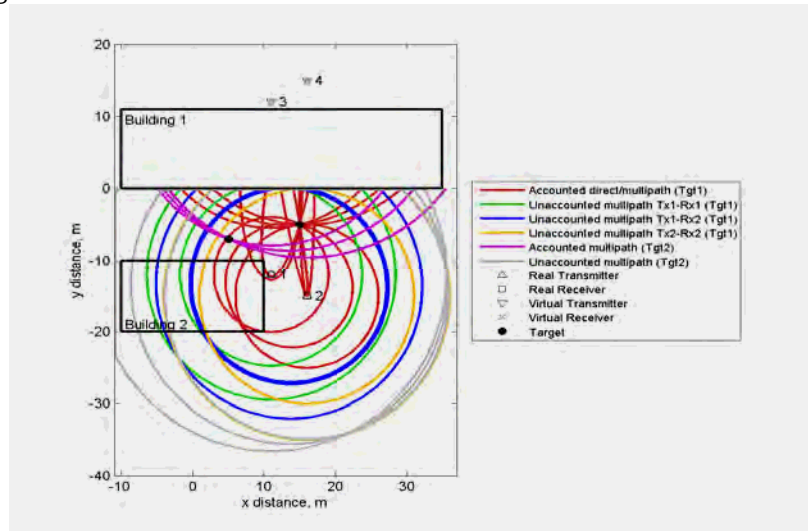
FIGURE 5. Ellipse geometry for two targets in a multipath environment using two Tx/Rx transceivers where there is no line-of-sight between one of the targets and the transceivers.
