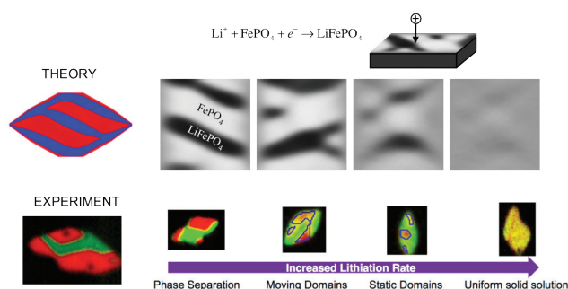
Figure 4: Phase separation patterns in lithium iron phosphate nanoparticles, which become suppressed with increasing discharge current. Top row: theoretical predictions. 11,14,15 Bottom row: subsequent experimental observations by in operando x-ray imaging from the group of W.C. Chueh. 18
