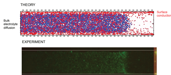
Figure 2: Theory 6 and experiments 7 on deionisation shocks.
