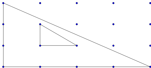
Figure 3: A polygon with a hole
