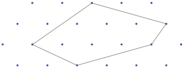
Figure 2: A polygon on a sheared lattice
